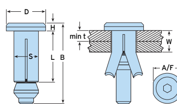
b) Countersunk
